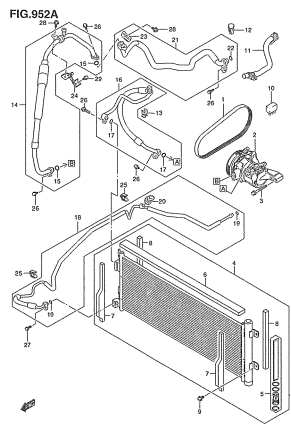
ZC33S R52A AIR CONDITIONER
