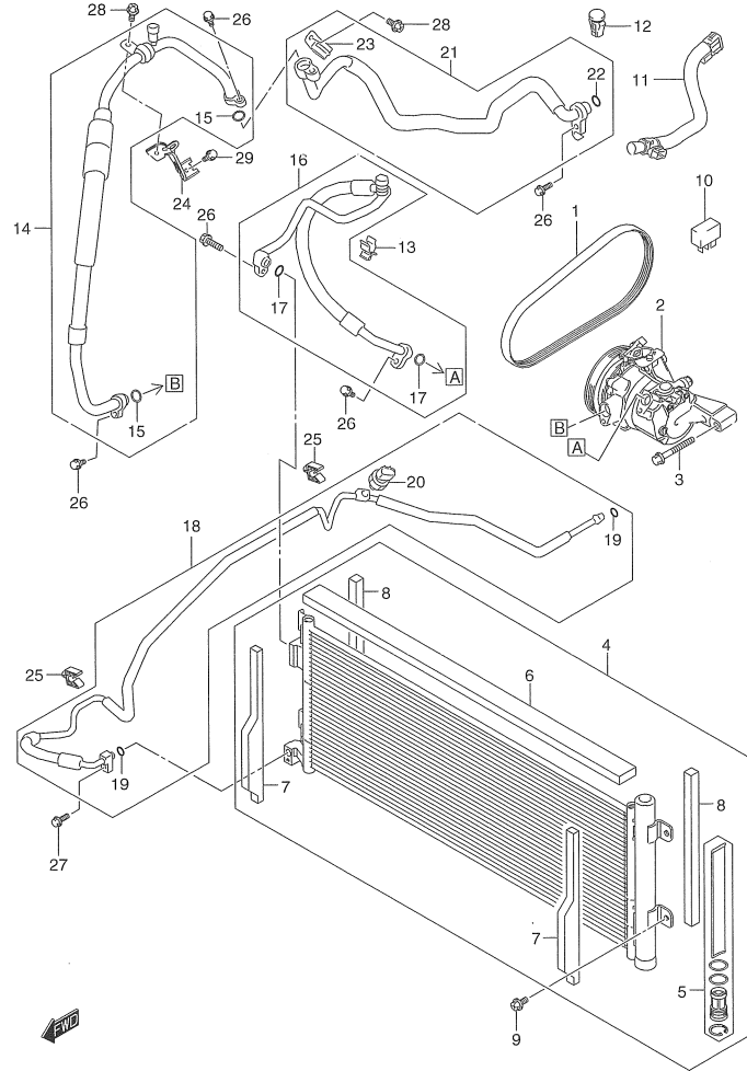
ZC33S 952A AIR CONDITIONER
