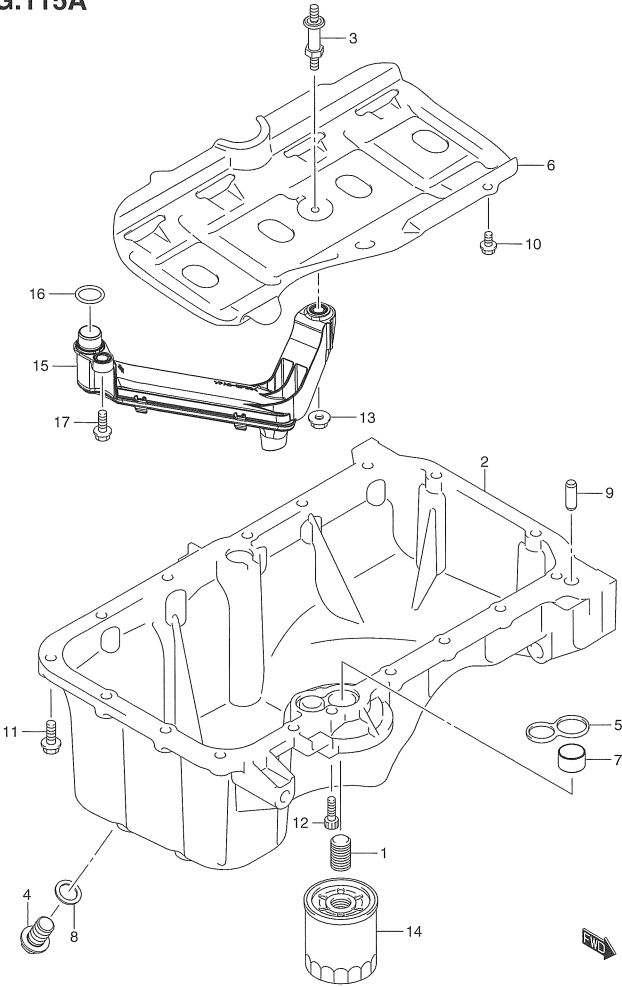
ZC33S 115A OIL PAN
