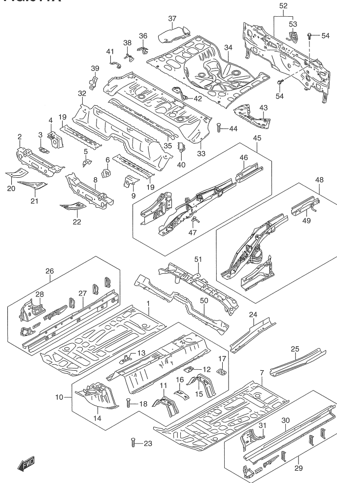
ZC33S 611A FLOOR PANEL
