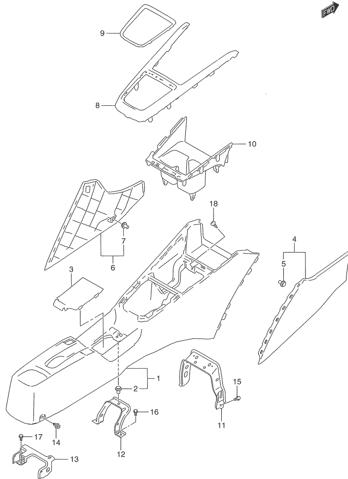
ZC33S 758A CONSOLE BOX
