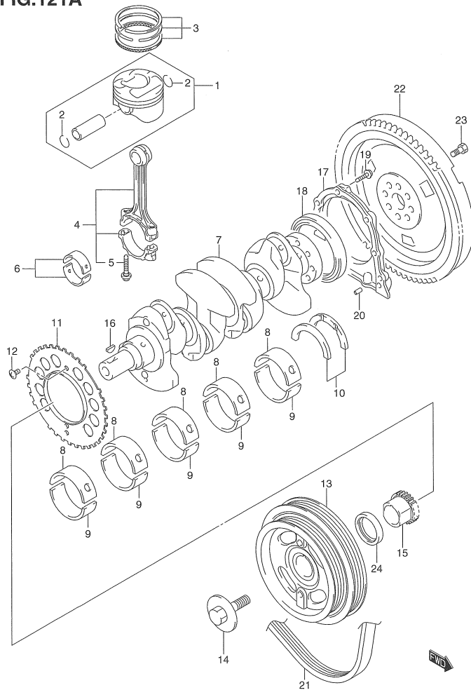
ZC33S 121A CRANKSHAFT
