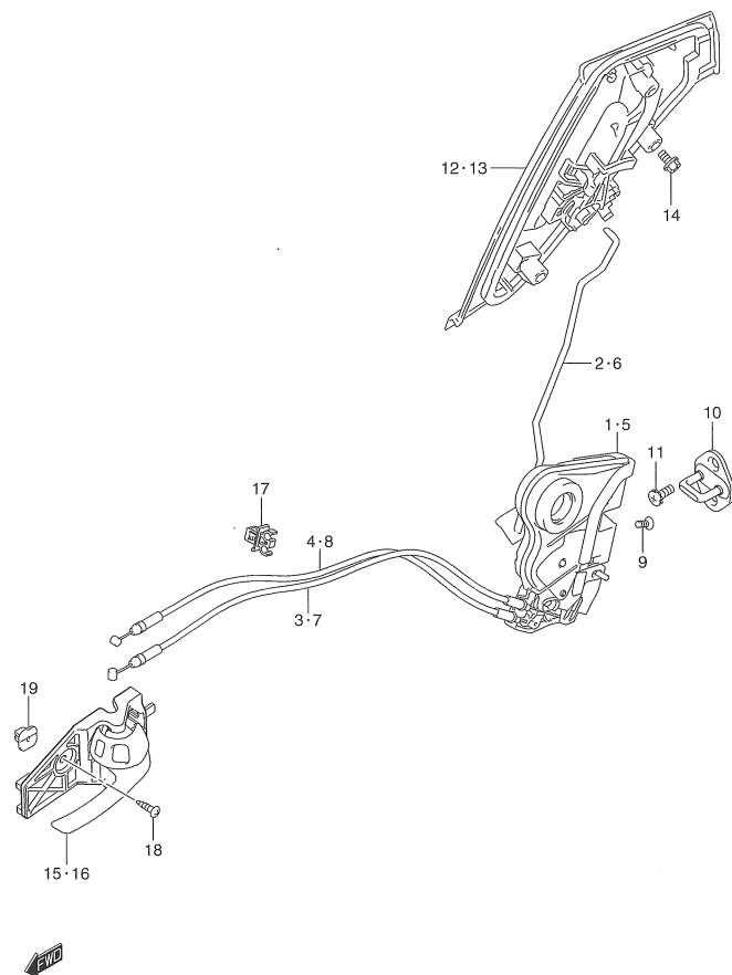
ZC33S 823A REAR DOOR LOCK
