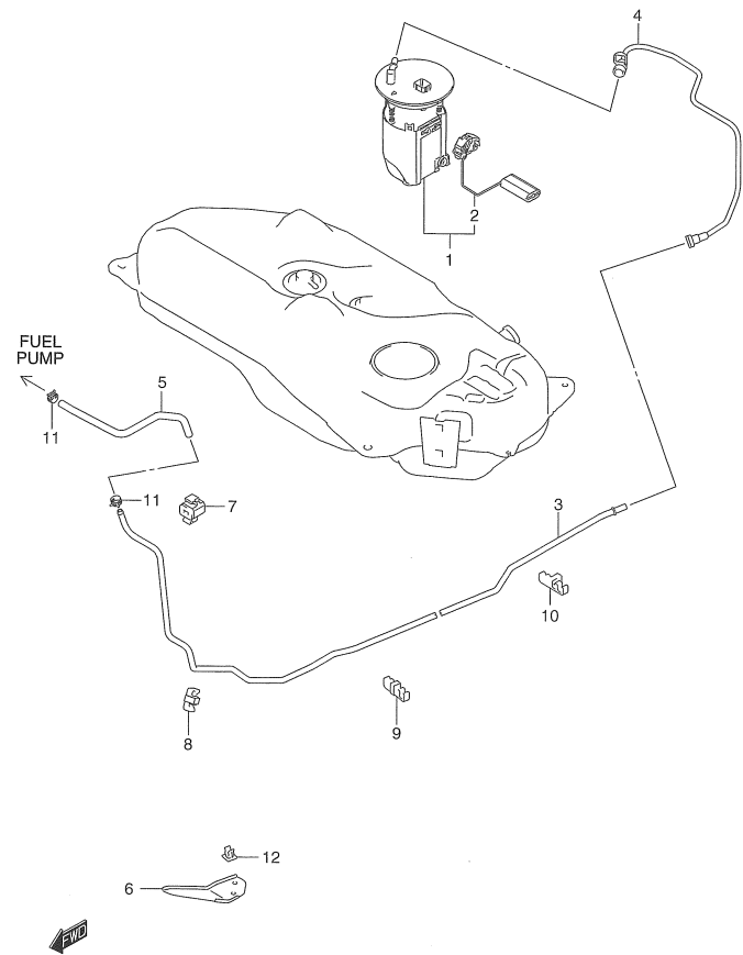
ZC33S 151A FUEL PUMP
