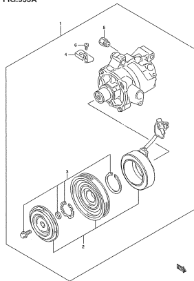
ZC33S R52A COMPRESSOR
