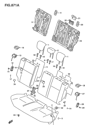
ZC33S 871A REAR SEAT
