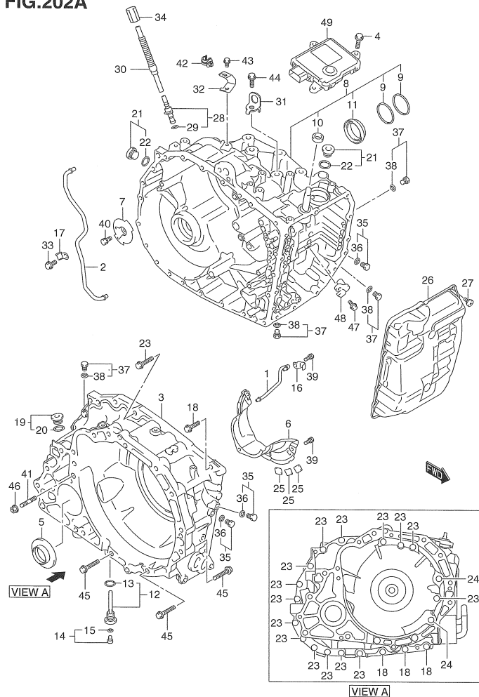
ZC33S 202A AT TRANSMISSION CASE
