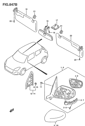
ZC33S 847B MIRROR/SUNVISOR (2)
