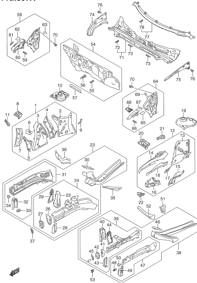
ZC33S 597A FRONT BODY PANEL
