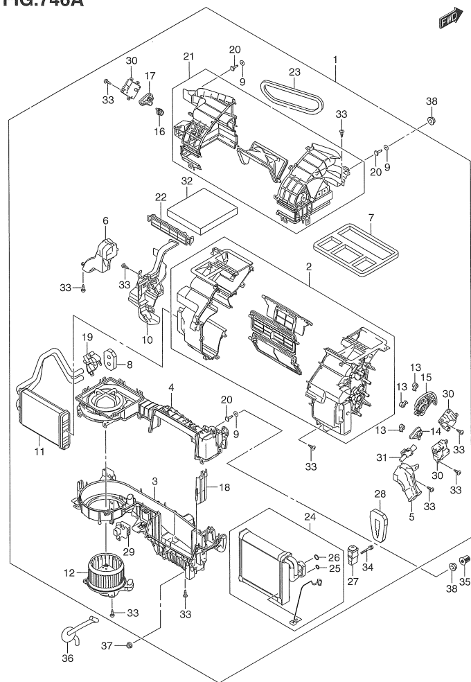
ZC33S 746A HEATER UNIT
