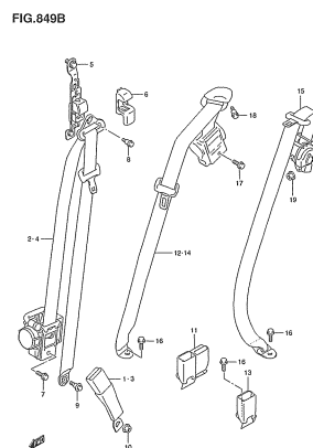
ZC33S 849B SEAT BELT (2)
