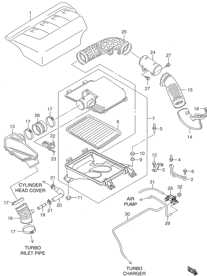
ZC33S 137A AIR CLEANER
