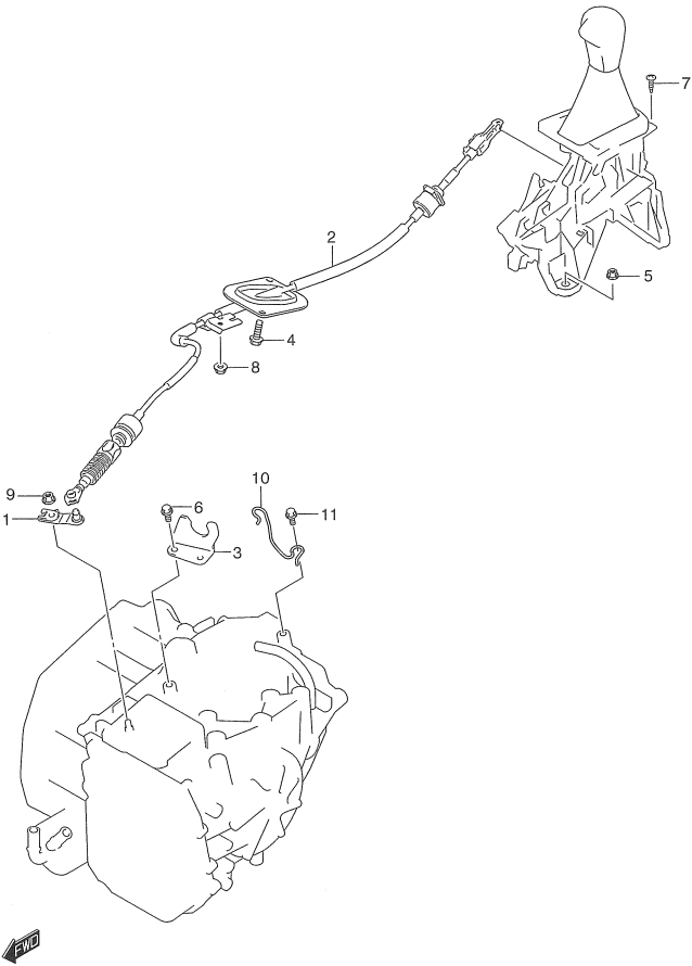
ZC33S 281B GEAR SHIFT CONTROL (2)
