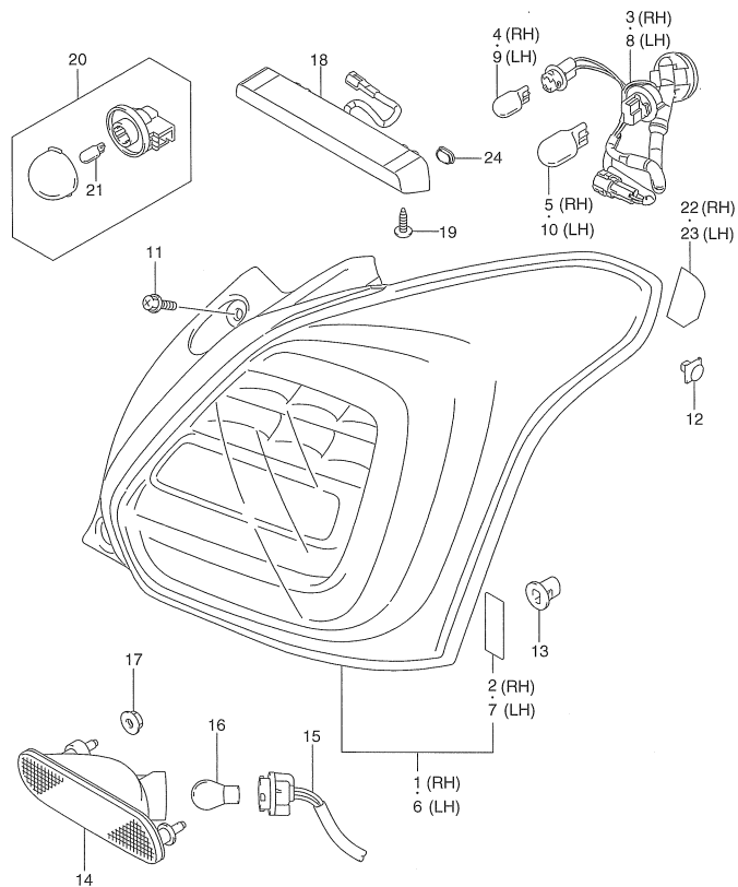
ZC33S 356A REAR LAMP
