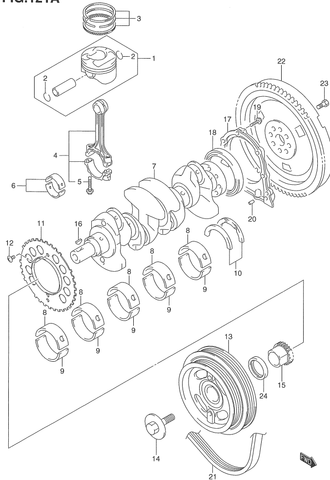
ZC33S 121A CRANKSHAFT
