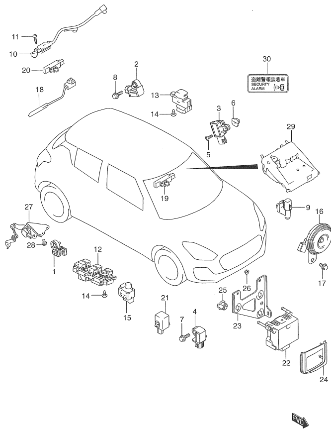
ZC33S 344A ELECTRICAL CONTROL BODY
