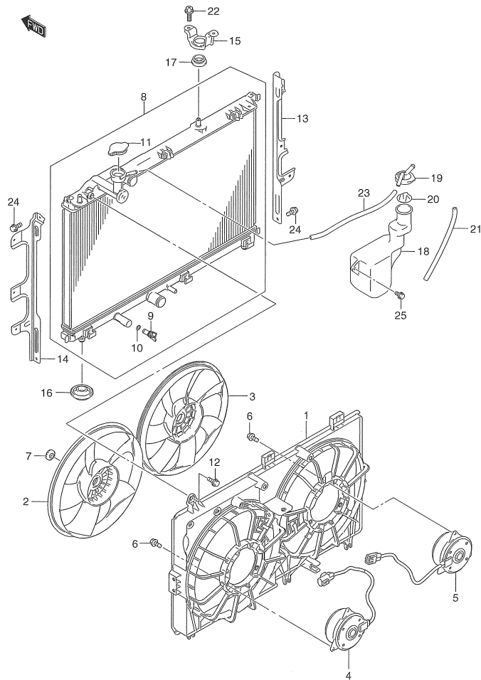
ZC33S 177A RADIATOR
