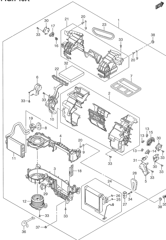
ZC33S 746A HEATER UNIT
